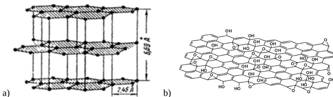
Figure 1. a) Crystal lattice of graphite. GO retains the layer structure of graphite, but the interlayer spacing is almost two times larger ( \sim 12 Å instead of 6.69 Å in the figure) and part of the carbon atoms are oxidized. b) Single sheet in the GO crystal lattice. Several oxygen containing functional groups are shown. Absolute and relative number of functional groups depends on the particular synthesis method.
